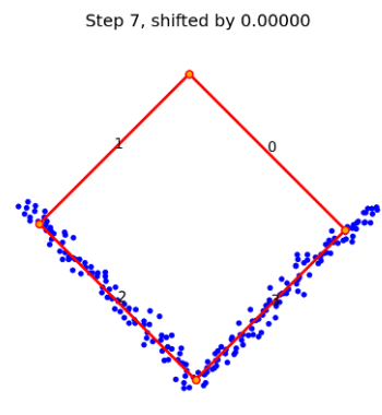
(e) \alpha = 1.00
