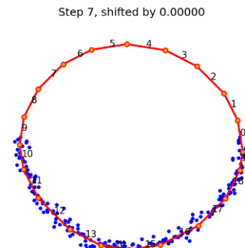
(e) \alpha = 1.00
