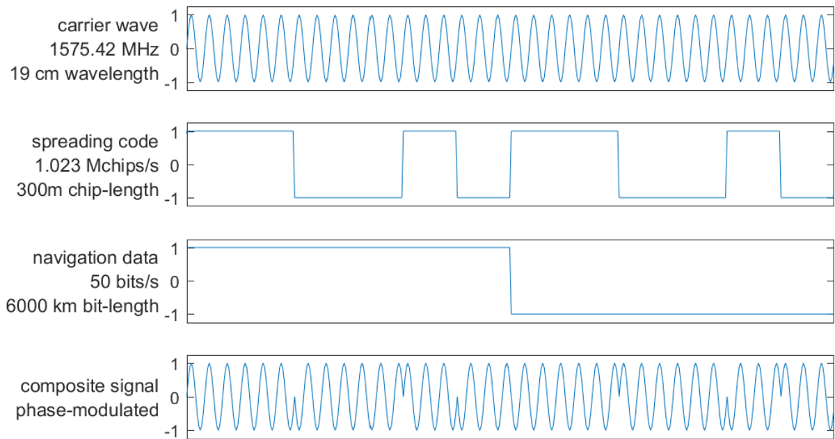
Figure 7: GPS L1 CA-signal (scale is not accurate)
