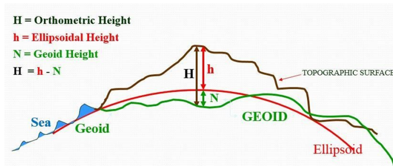
Figure 17: Physical heights in Geomatics
