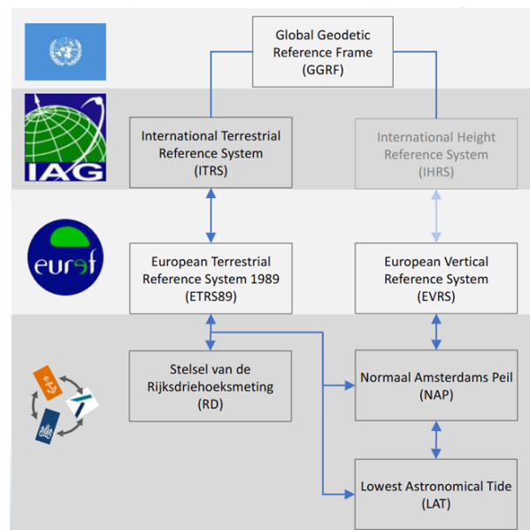
Figure 14: Terrestrial Reference Systems
