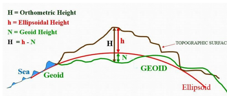
Figure 17: Physical heights in Geomatics
