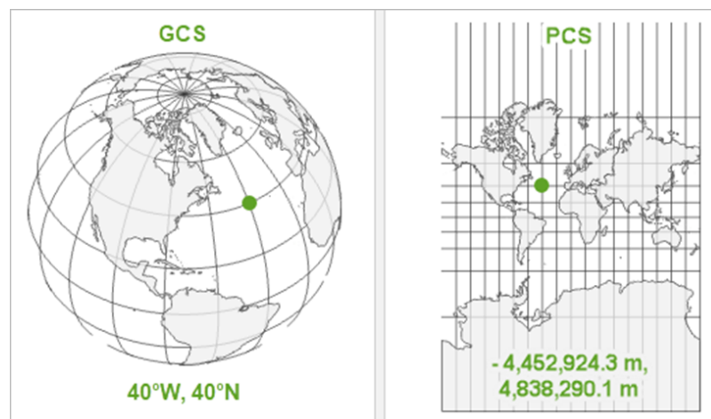
Figure 12: Geographic coordinate systems vs Projected coordinate system
