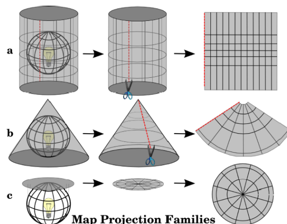
Figure 18: Map Projection Families
