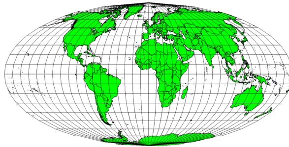
Figure 21: Equal area map projection
