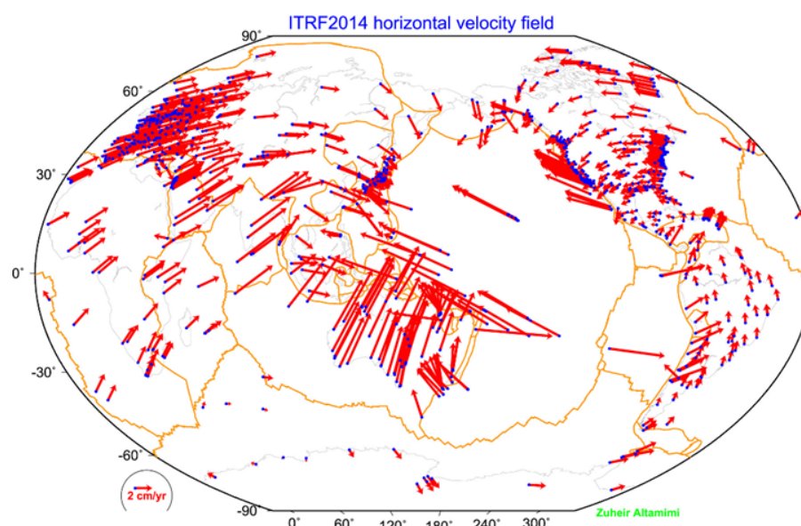
Figure 15: Changes in ITRF2014
