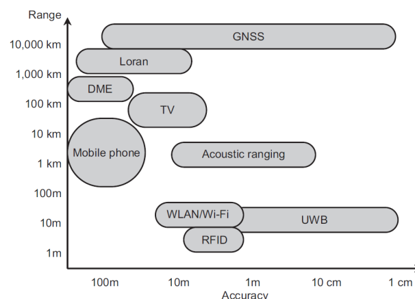
Figure 1.13 Range and accuracy of signal-based positioning technologies.
