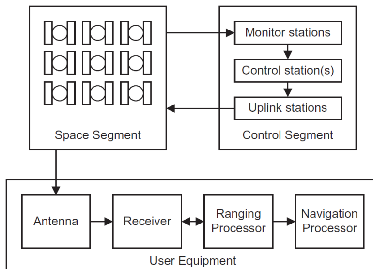
Figure 5: GPS segments
