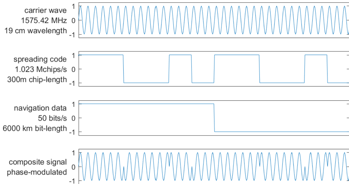
Figure 6: GPS L1 CA-signal (scale is not accurate)
