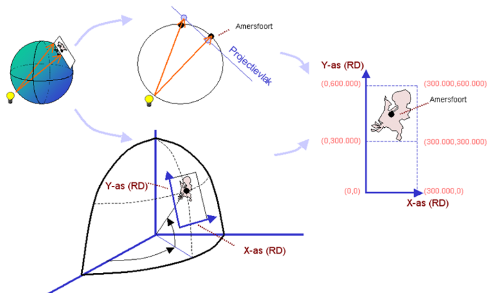
Figure 22: RDNAP diagram
