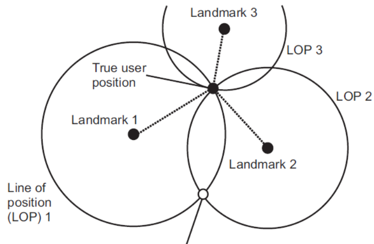
Figure 1.8 Positioning by ranging in two dimensions.
