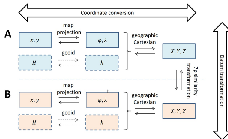
Figure 16: Map of coordinate conversion and datum transformation
