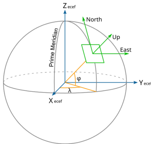
Figure 11: Fundamentals of a Geographic coordinate system
