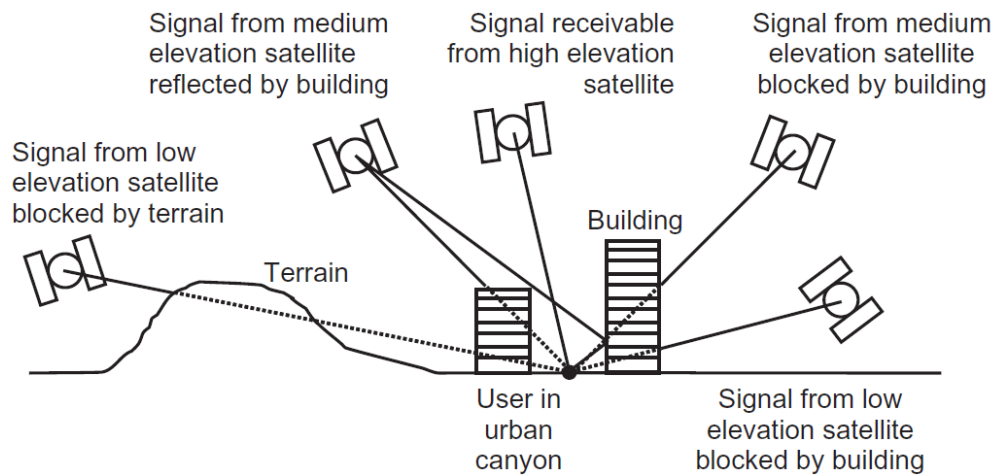
Figure 7: Errors due to terrain, buildings, and elevation angle
